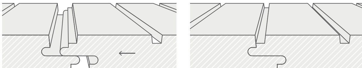
Invisilock™ Join
